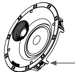
Figure 2: Roto-Lock Toggle Feet Retracted
